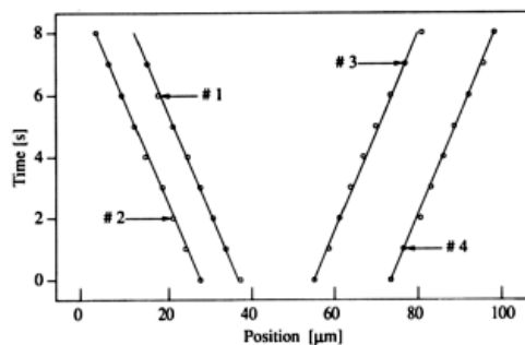
FIG. 2. Variation with time of the position of the solitary waves marked in Fig. 1 along their respective axis of propagation. The slopes yield a velocity of v = \pm 3.2 \mu\text{m/s} .
