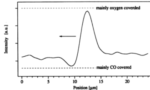
FIG. 3. (Negative) intensity profile of a solitary wave along its direction of propagation.
