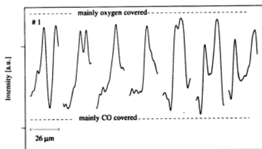
FIG. 5. Intensity profiles along the propagation direction from the PEEM images displayed in Fig. 4.
