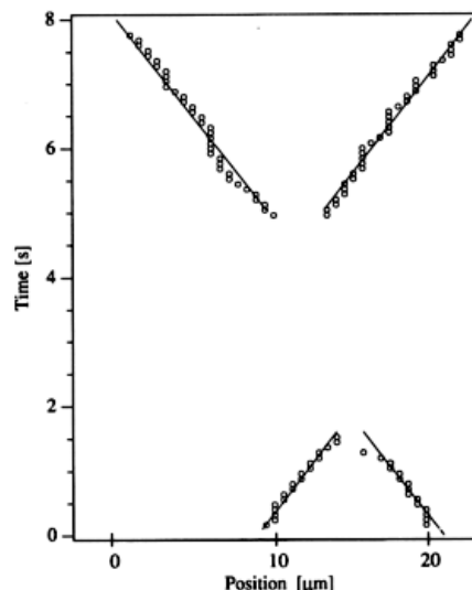
FIG. 6. Position of the intensity maxima of the two pulses of Fig. 4 as a function of time. The central region marks the collision zone which continues to propagate; hence there is no direct continuation of the straight lines in the lower and upper parts.
